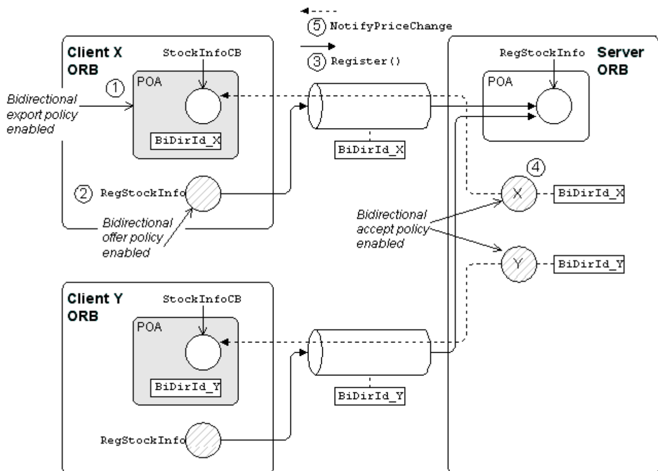
Figure 61 Basic Bidirectional GIOP Scenario—Stock Feed
