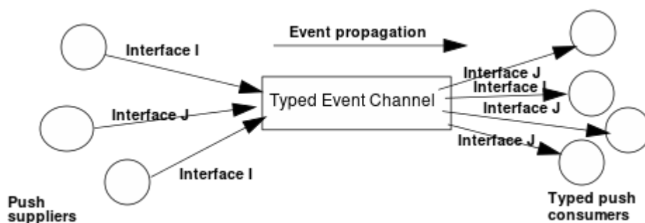
Figure 51 Push consumers pushing typed events to typed push consumers
