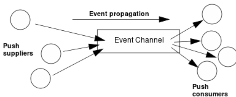
Figure 48 Push model of event transfer
