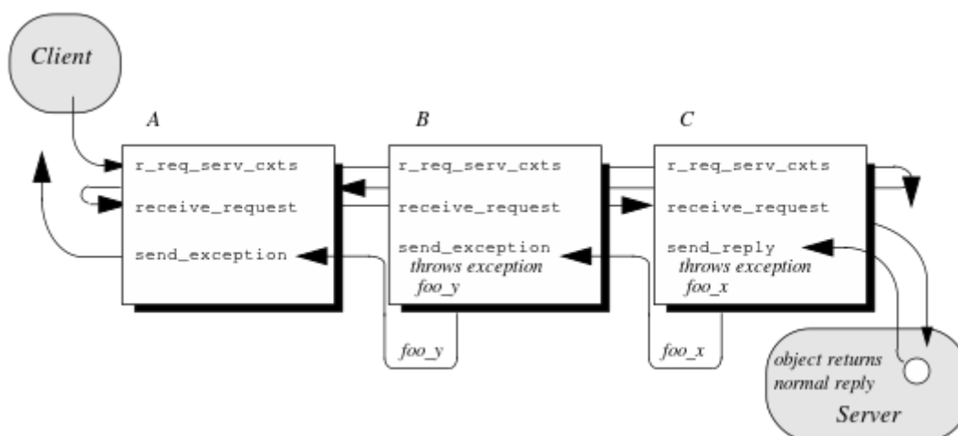
Figure 60 Server interceptors can change the reply type.
