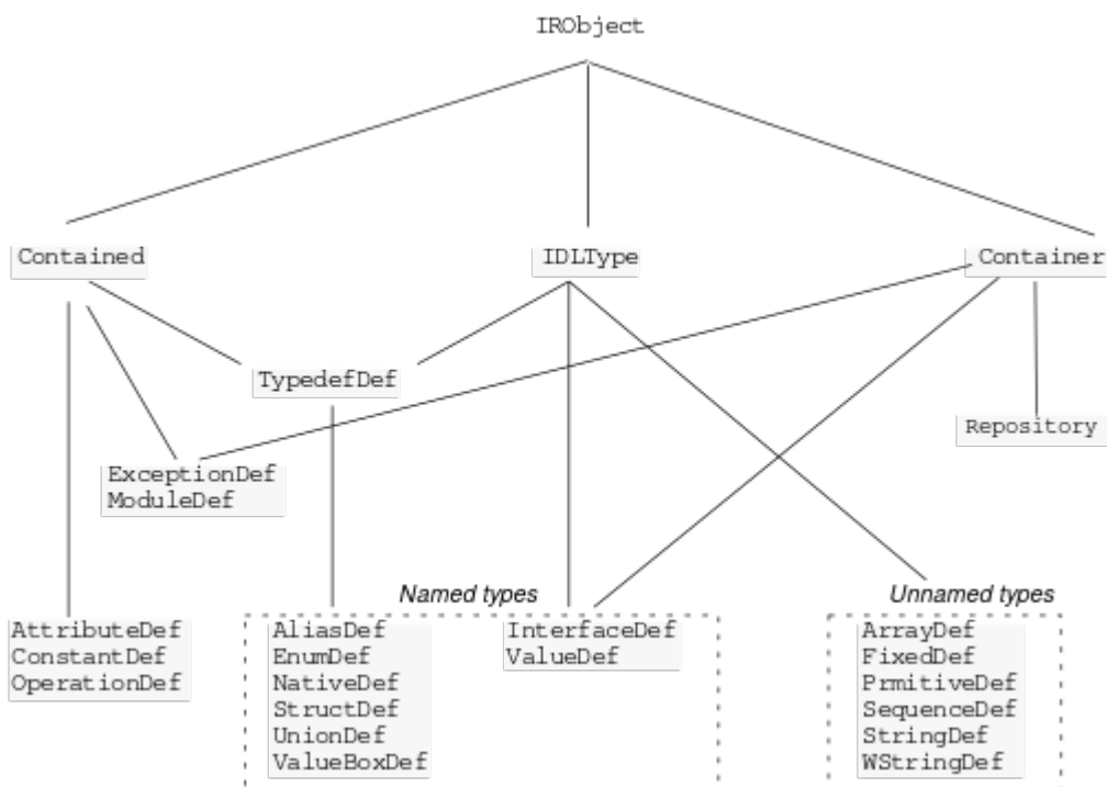
Figure 30 Hierarchy of interface repository objects
