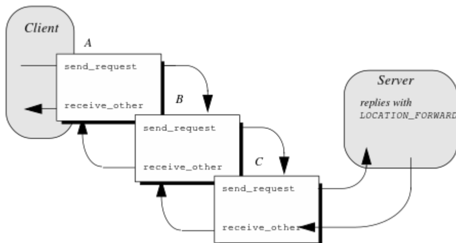
Figure 55 Client interceptors process a LOCATION_FORWARD reply.
