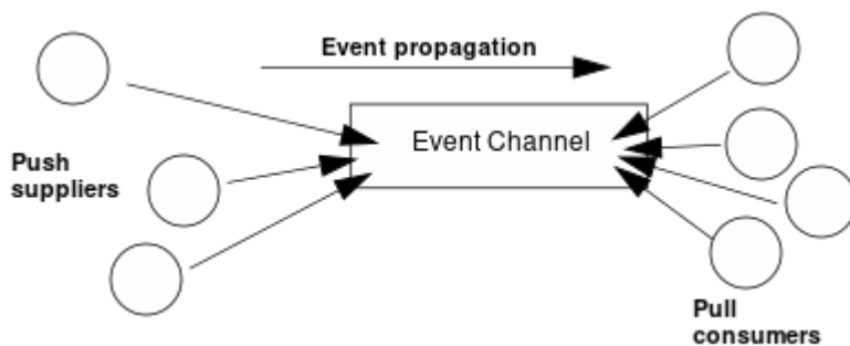
Figure 50 Push suppliers and pull consumers communicating through an event channel
