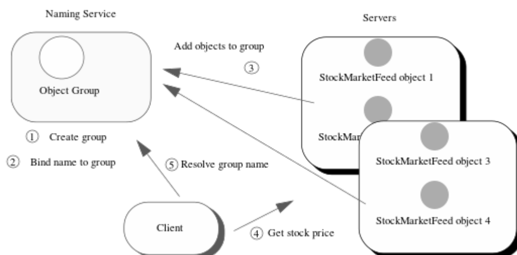
Figure 40 Architecture of the stock market example
