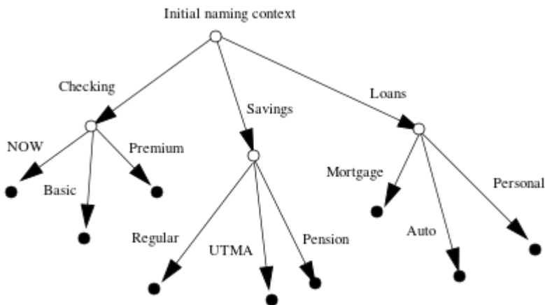
Figure 31 A naming graph is a hierarchy of naming contexts
