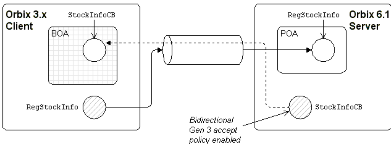
Figure 63 Orbix 3 Client Receiving a Callback from an Orbix 6.1 Server
