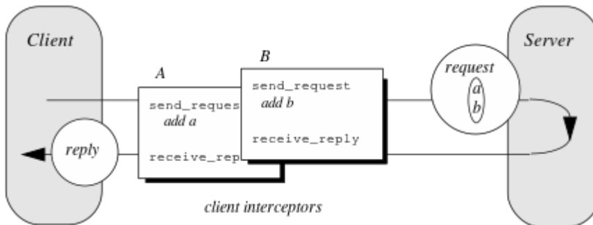
Figure 52 Client interceptors allow services to access outgoing requests and incoming replies.
