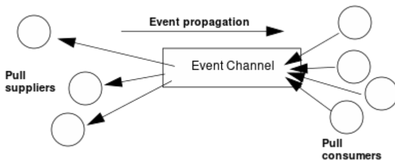
Figure 49 Pull Model suppliers and consumers communicating through an event channel
