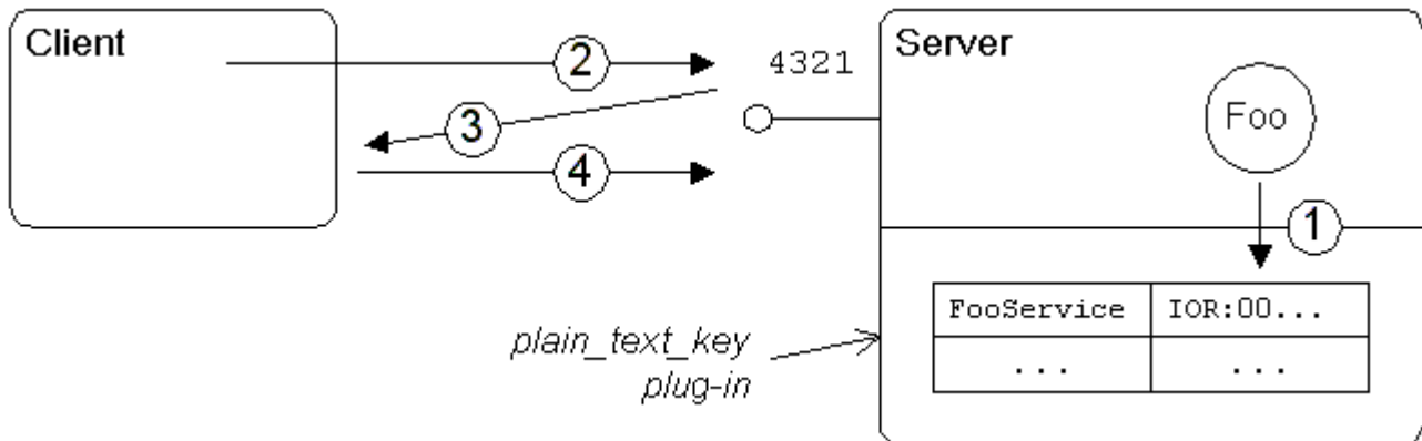
Figure 65 Using corbaloc with the plain_text_key Plug-In
