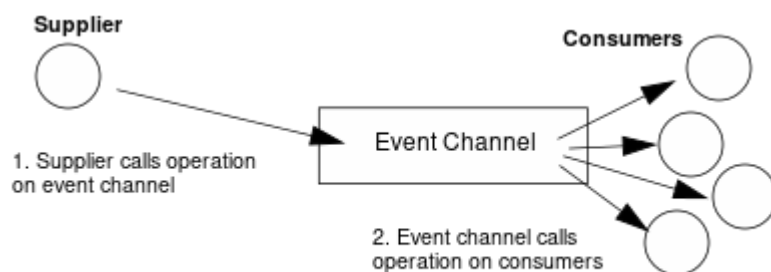
Figure 47 Event propagation in a CORBA system
