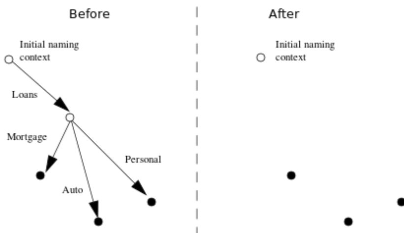
Figure 35 Destroying a naming context and removing related bindings
