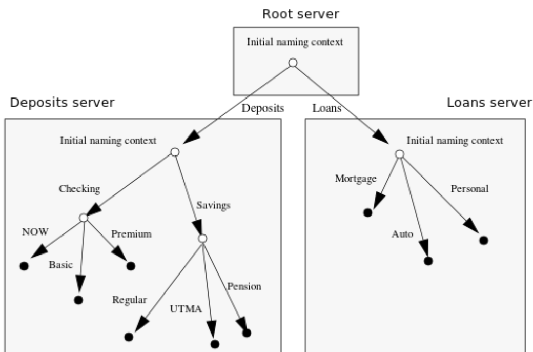
Figure 36 A naming graph that spans multiple servers
