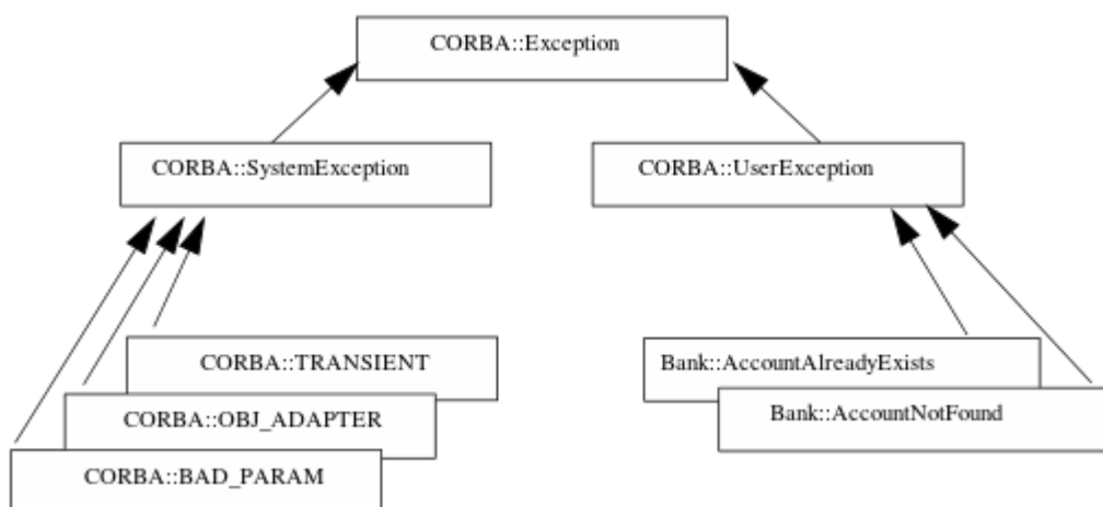
Figure 28 The C++ mapping arranges exceptions into a hierarchy
